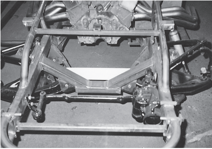
Small Block Supermodified using full fabricated frame.
