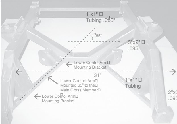
Small Block Supermodified using full fabricated frame.
